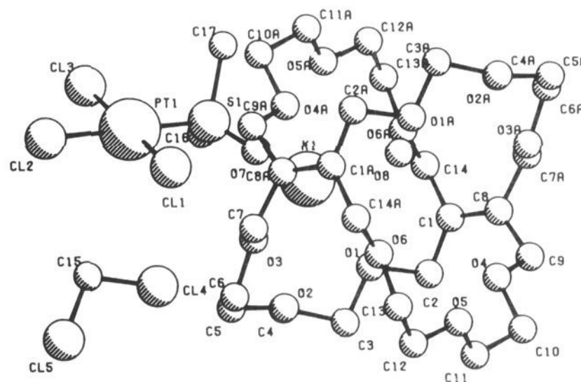
Figure 5. Perspective view and numbering scheme for complex 7 · CH_2Cl_2 . The [PtCl_3DMSO]^- anion, the K^+ cation, and the H_2O molecule within the cage are shown in only one symmetry position for clarity. Atoms labeled A have been generated by the symmetry operation -x, -y, -z .
