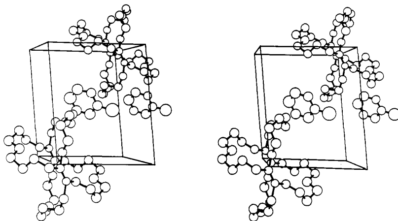
Figure 2. Unit cell diagram for cage 5 -toluene.
